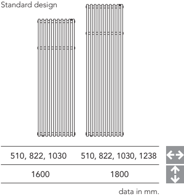
VELINO model: Standard design
