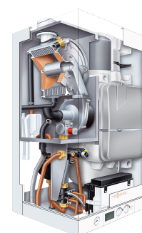
Vitodens 111-W Showing Internal Components
